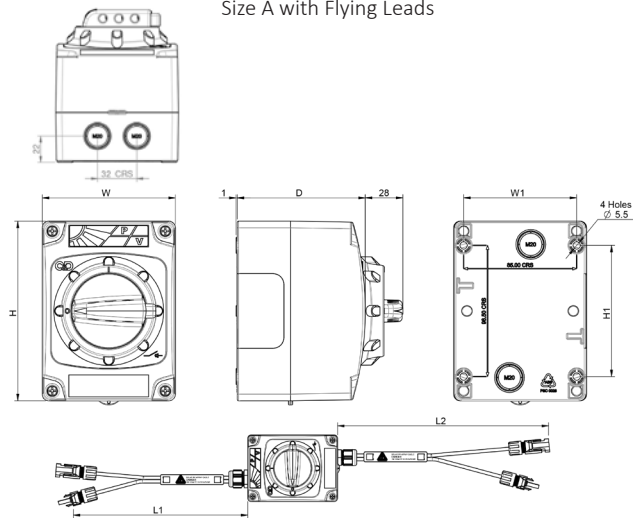
Size A with Flying Leads
