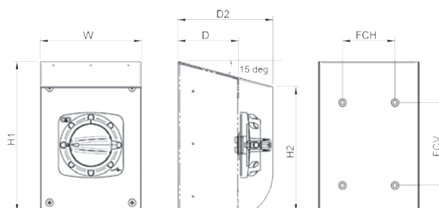
Size A & B
