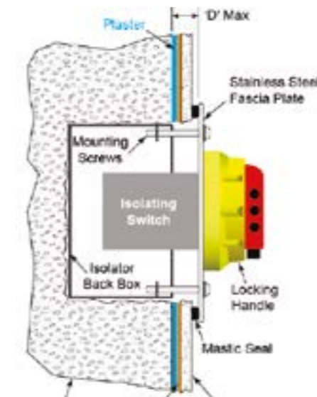
Typical Installation 'D' max = 20mm with standard length mounting screws
