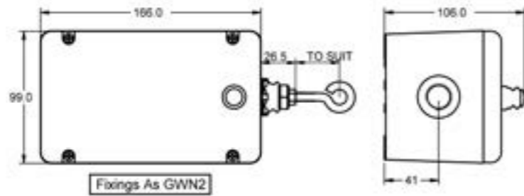
GW/AB Anchor Box
